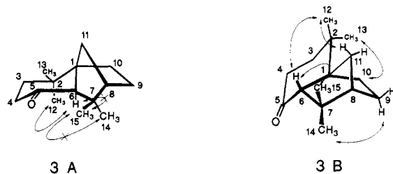
Figure 2. Two epimers of isolongifolene ketone 3 showing the NOE cross-peaks.
